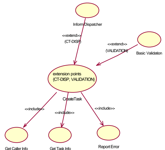
Figure 10. A customized Create Task use case
