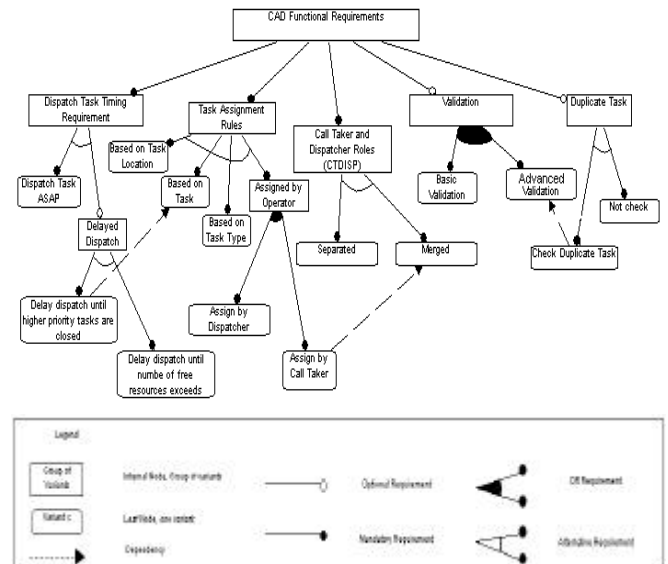
Figure 3. CAD feature model
