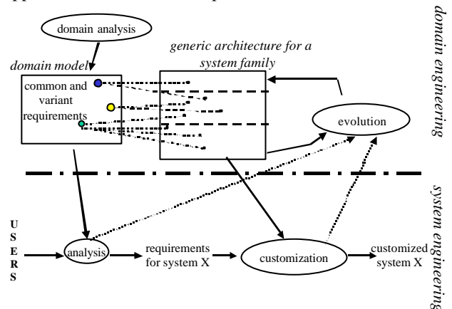
Figure 1. Domain and system engineering
