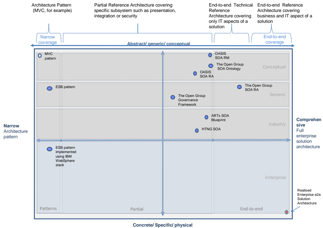
Figure 21: SOA Standards
