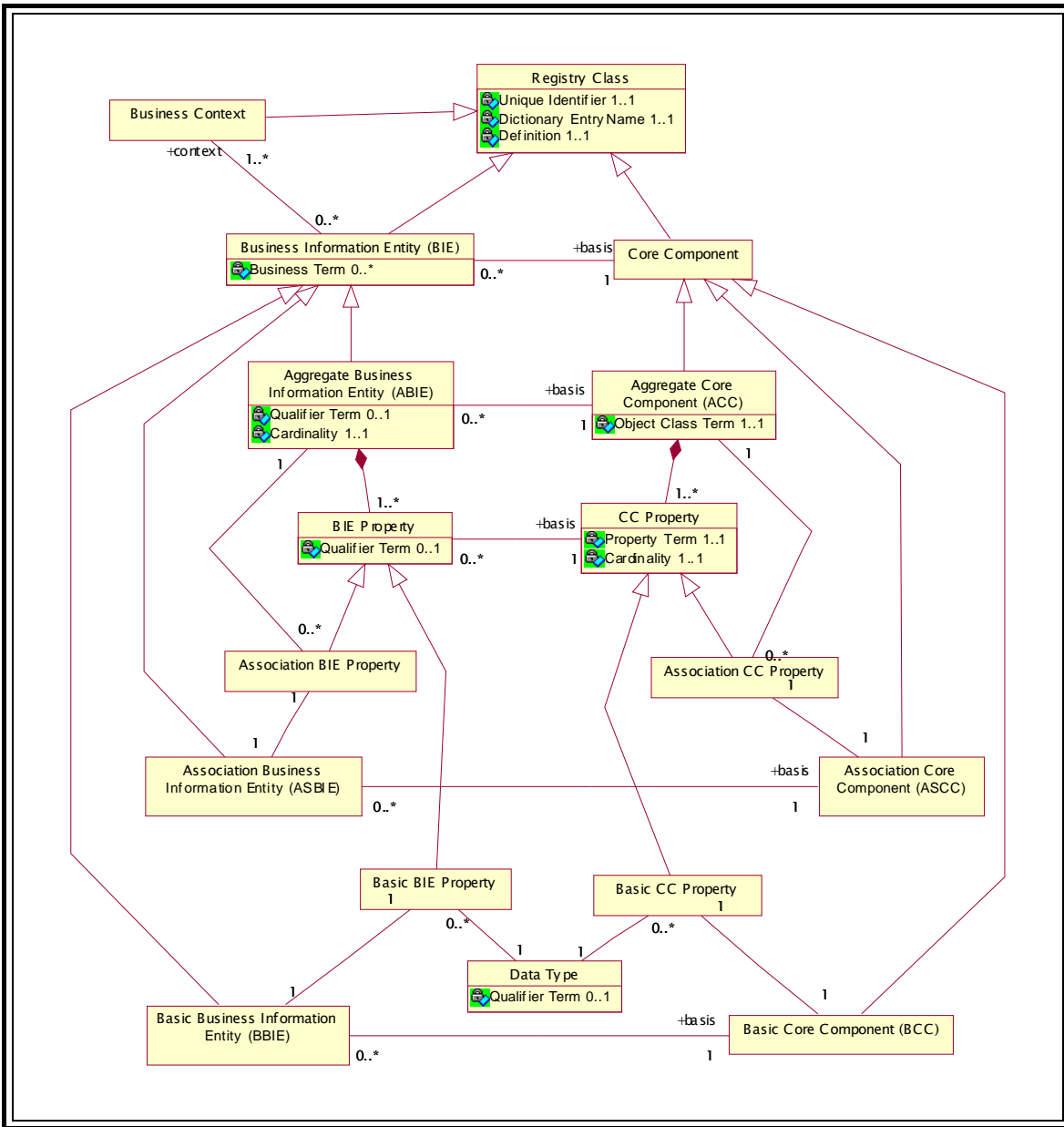
Figure 5-2 Context Specific Business Information Entity Metamodel
