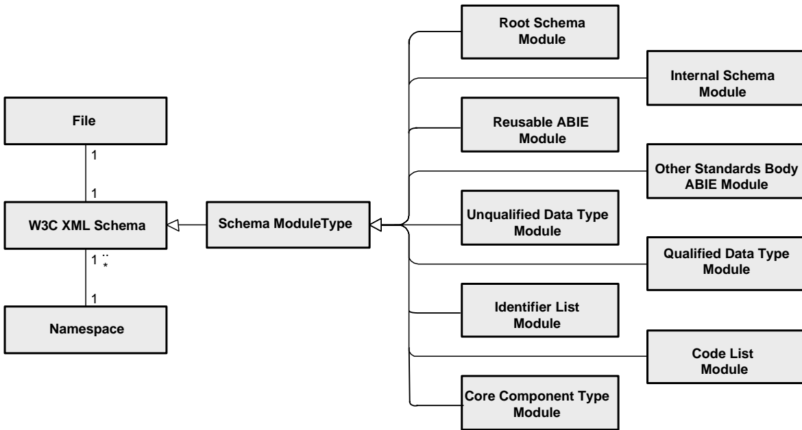
550 Figure 5-5 UN/CEFACT XSD Schema Modules
