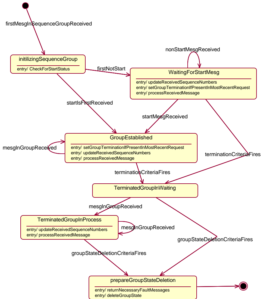
Figure 1 – State Machine for Messages in Sequence Group
