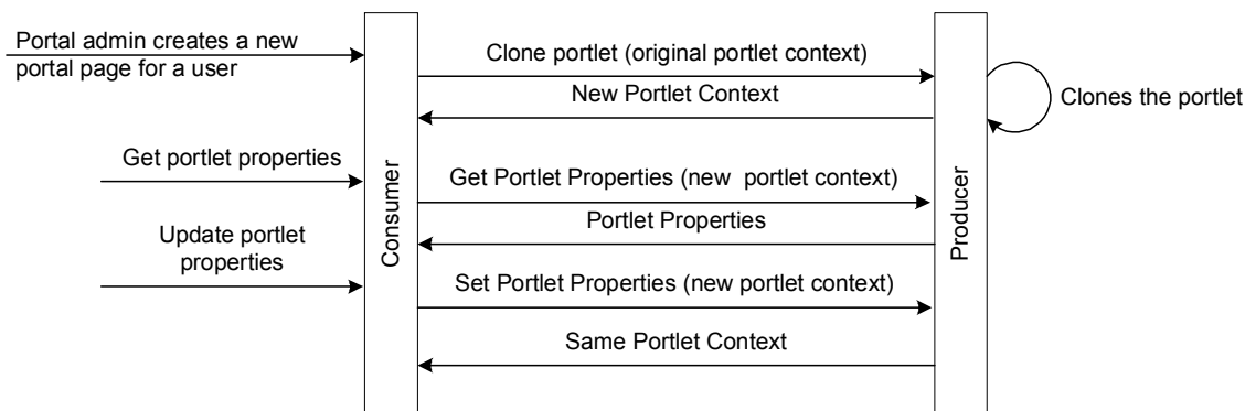
Figure 6: Cloning and Setting Portlet Properties
