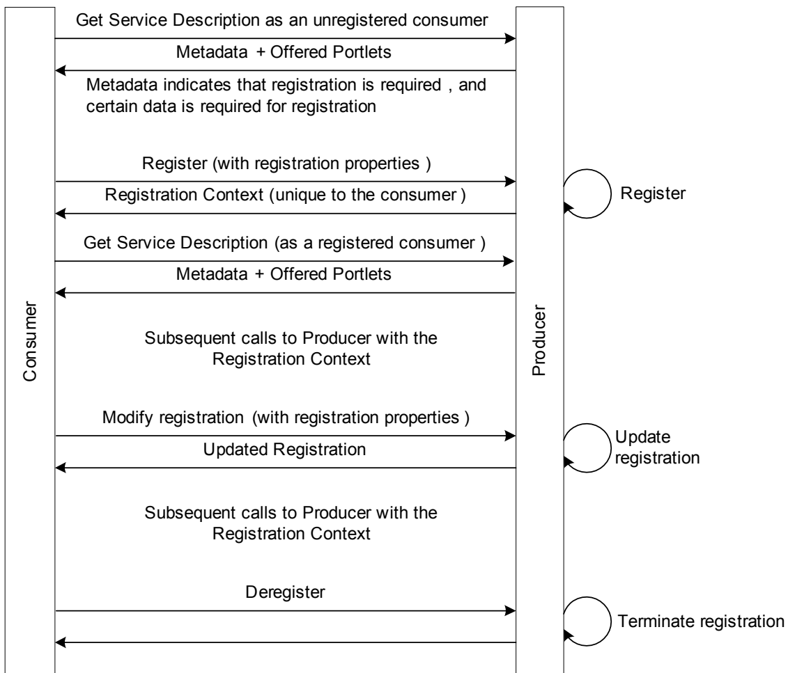
Figure 2: Registration Impact on Consumer-Producer Interactions
