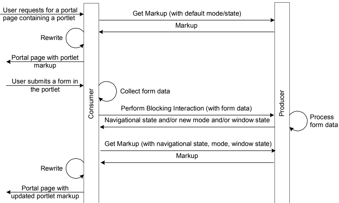
Figure 3: Two Step Protocol
