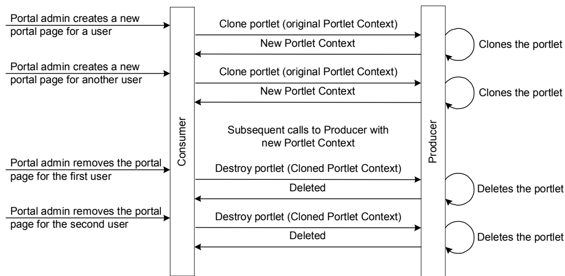
Figure 7: Cloning and Destroy for Managing Portlet Customizations
