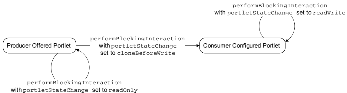
Figure 4: Persistent Lifecycle of Portlets with Implicit Cloning
