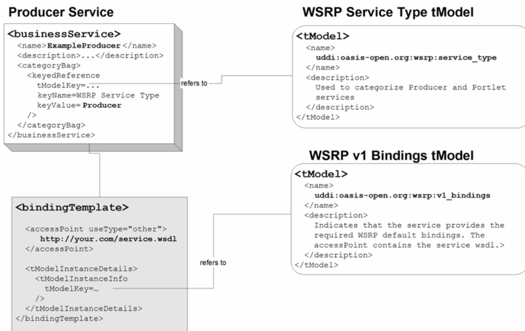
Figure 2: Publishing Producers
