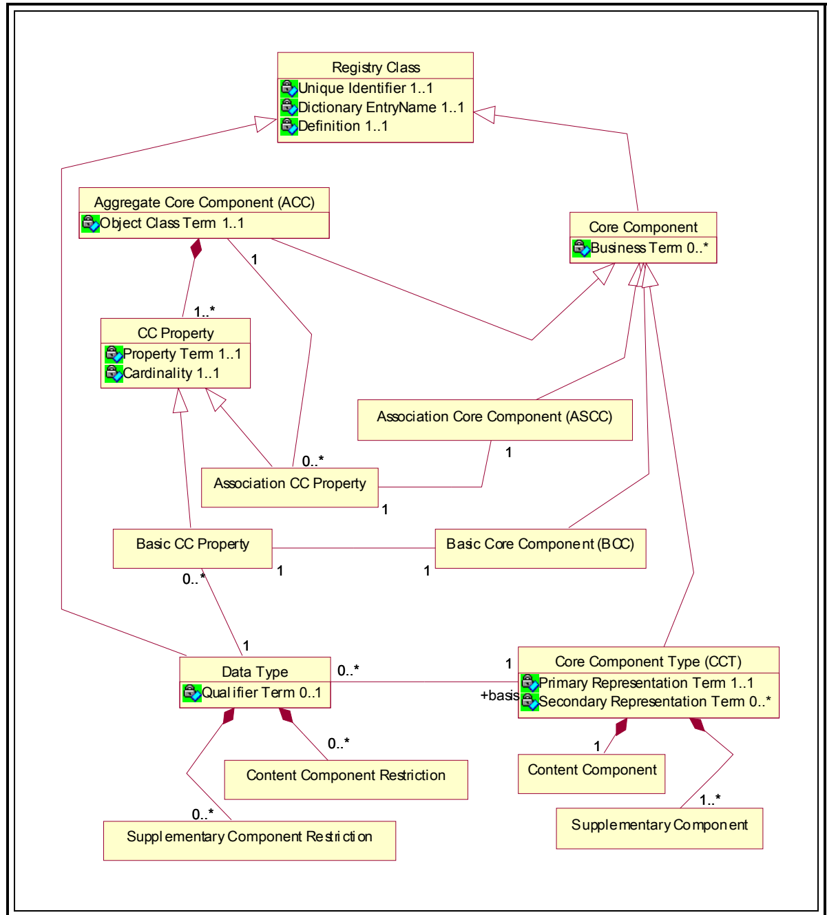
Figure 6-1. Core Components and Data Types Metamodel
